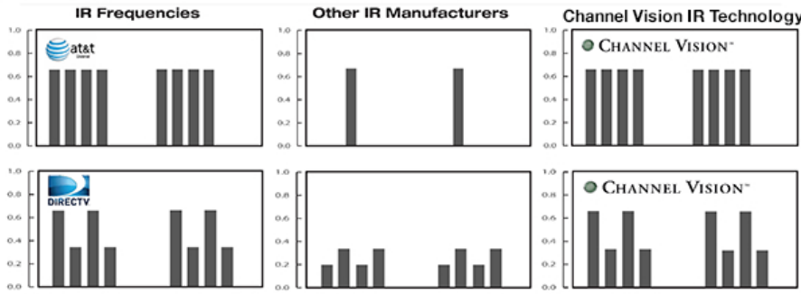
Frequency levels of Channel Vision's Uverse® Ready, IR Repeater Systems compared to other IR systems using AT&T Uverse® cable boxes.
